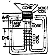
Electrodynamic loudspeaker.
